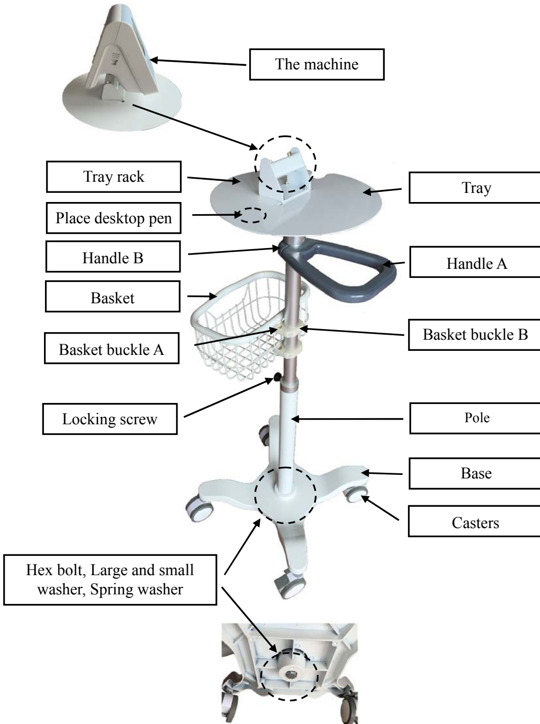
Figure 1 BVT01-YZT-3B Trolley parts diagram
